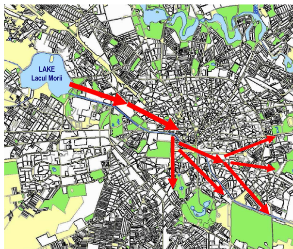
Fig. 4. Flooding scenario from Lake Lacul Morii, having impact on study area and beyond (Project URBASRISK, 2014-2015)
