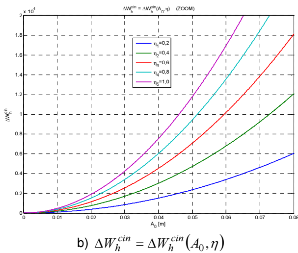
Fig. 7. Family of curves for the dissipated energy for [V] and [H] models
