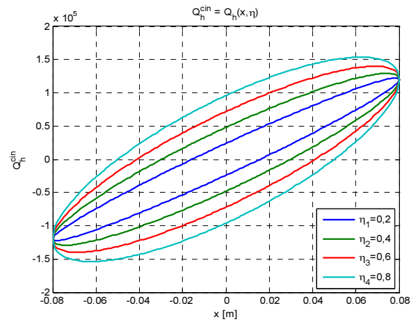
Fig. 5. Hysteresis curve
