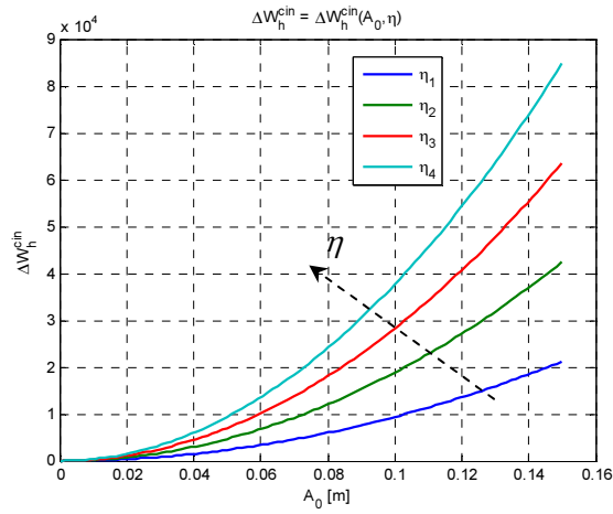
Fig. 3. Dissipated energy
