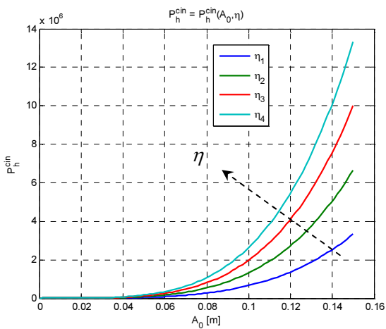
Fig. 4. Dissipated power
