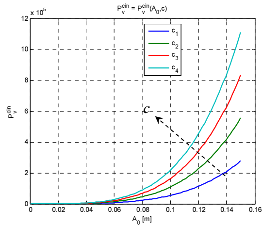
Fig. 3. Dissipated energy
