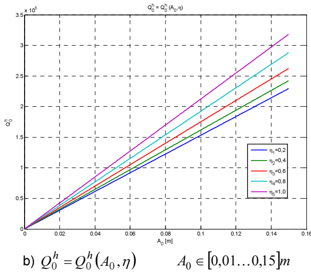
Fig. 6. Family of curves for the reaction forces for [V] and [H] models
