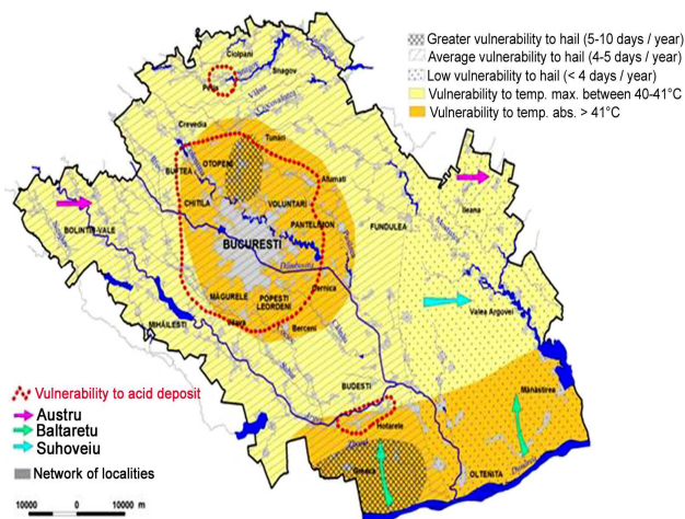
Fig. 11. Map with climate hazards – Bucharest, summer season
