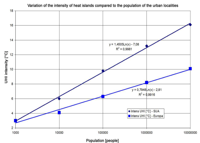
Fig. 6. Intensity of urban heat islands compared to the population
