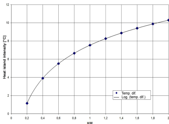
Fig. 7. Correlation of the intensity of urban heat islands with the geometrical characteristics of the urban environment
