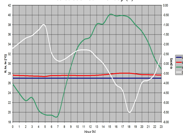
Fig. 24. Thermal regime – artificial air conditioning a)
