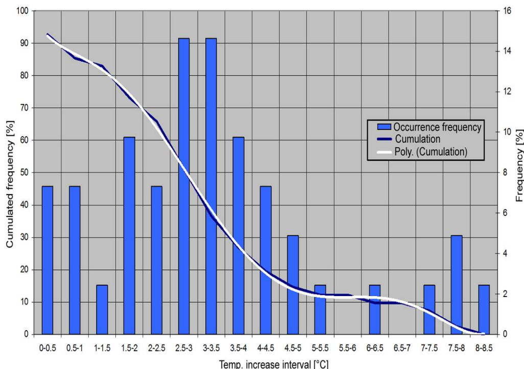
Fig. 1. Statistics of the increase in average outdoor temperature of the coldest pentad in 41 localities in Romania during 1994-2008 compared with the period 1961-1994 (Climate 2 compared to Climate 1)
