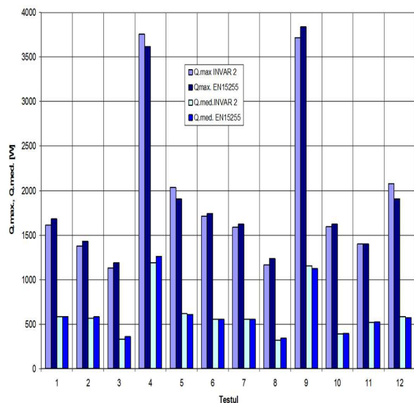
Fig.17. rQ indicator, test synthesis 1...12
