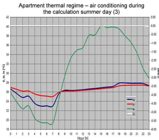
Fig. 28. Thermal regime – artificial air conditioning c)
