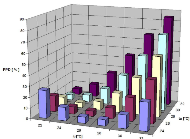
Fig. 8. Variation of the PPD index depending on the indoor air and radiant mean temperature
