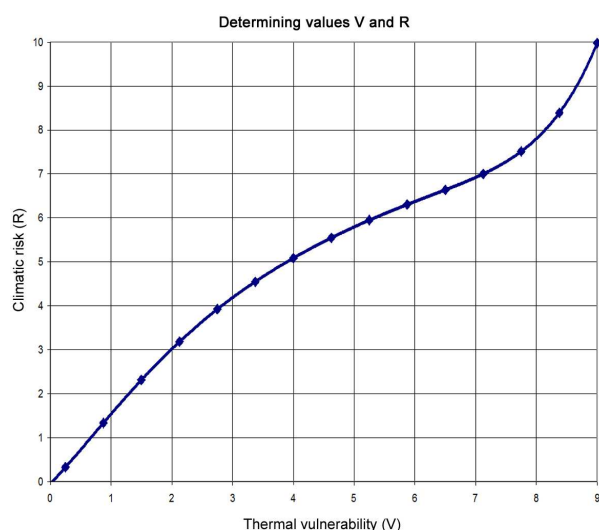
Fig. 9. Variation of climatic risk ( R ) depending on the thermal vulnerability ( V ) of the buildings
