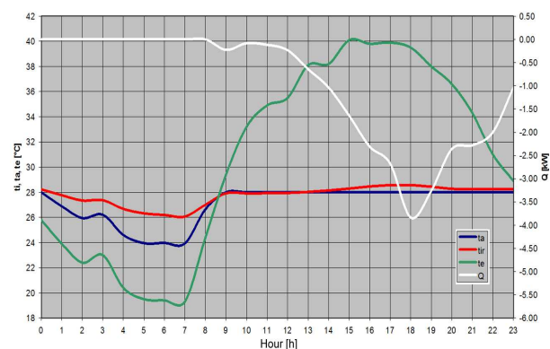
Fig. 26. Thermal regime – artificial air conditioning b)
