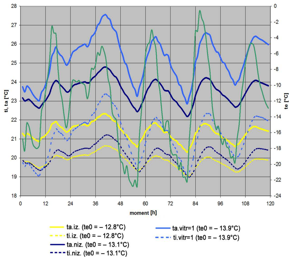
Fig. 3. Case study – Bucharest, extreme calculus climate 2 (1994-2008) (non-isolated cover / thermally isolated cover and double/thermo-isolating windows) – corner premises
