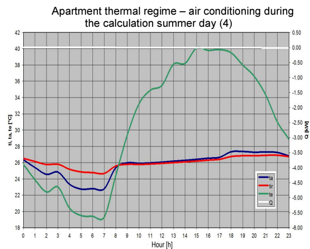
Fig. 30. Thermal regime – artificial air conditioning d)
