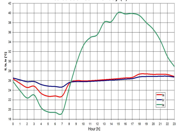
Fig. 29. Natural thermal regime – status d)
