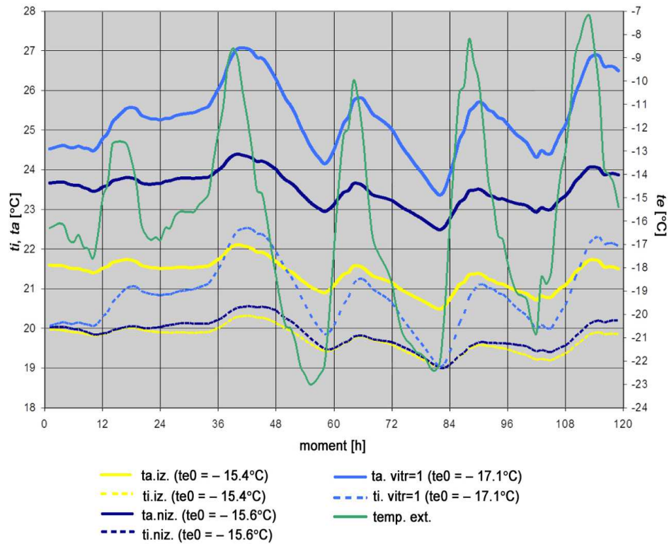
Fig. 2. Case study – Bucharest, calculus climate 1 (1961-1994) (non-isolated cover / thermally isolated cover and double / thermo-isolating windows) – corner premises
