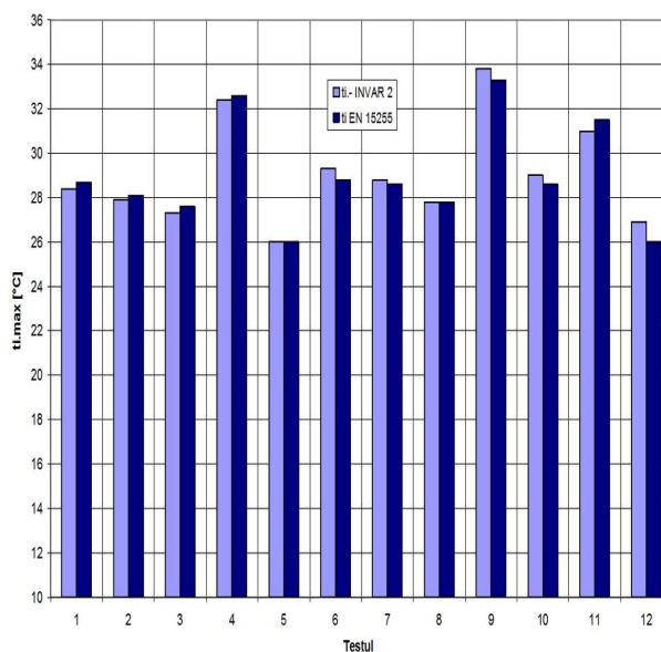
Fig. 18. r\vartheta_i indicator, test synthesis 1...12
