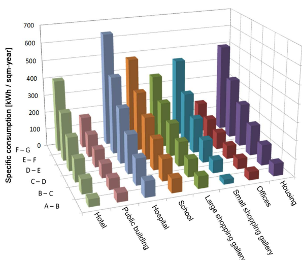
Fig. 12. Energy classes for heating
