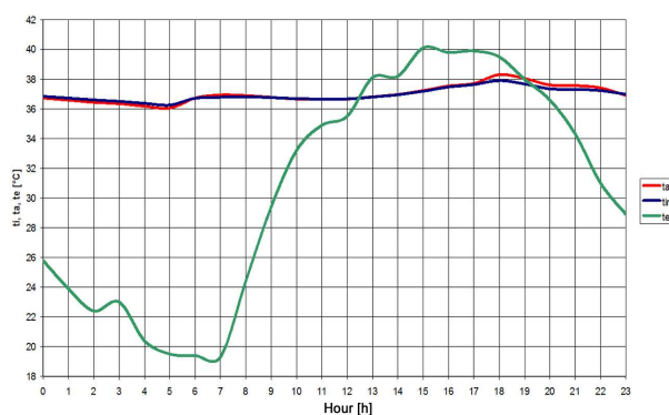
Fig. 23. Natural thermal regime – current status a)
