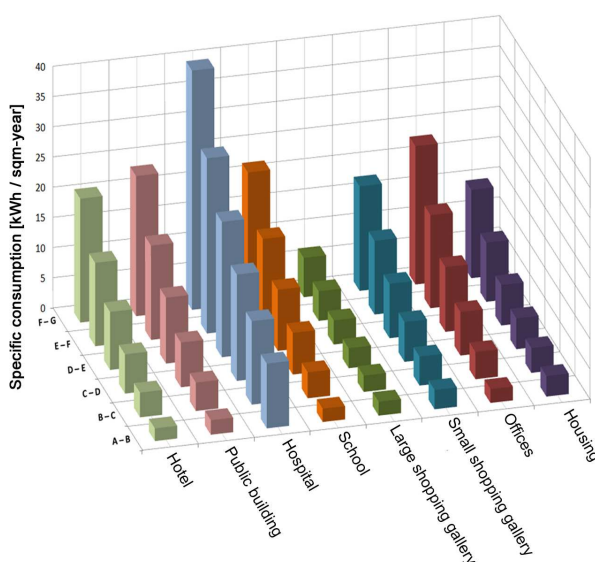
Fig. 13. Energy classes for space air conditioning
