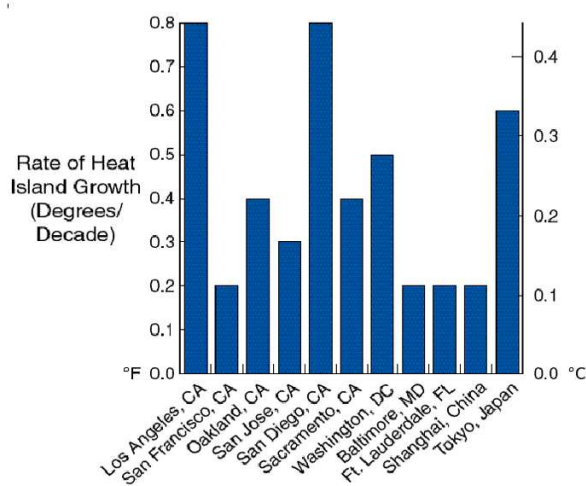
Fig. 4. Dynamic of the increase in urban heat islands
