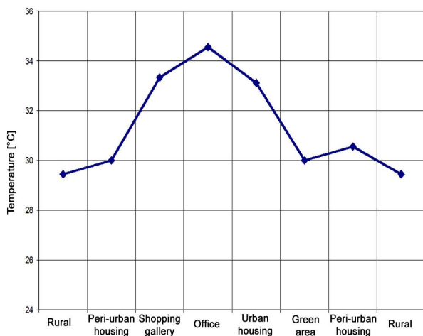
Fig. 5. Profile of an urban heat island
