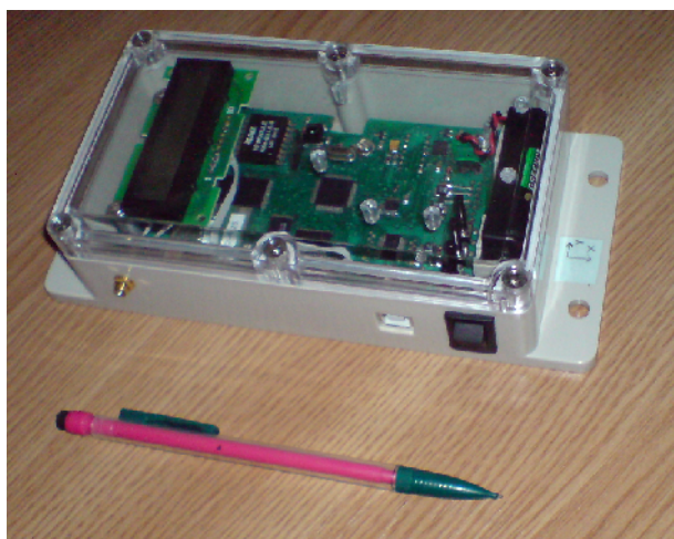
Figure 20. MEMS-based data logger
