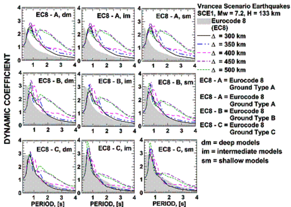
Figure 12. Vrancea scenario earthquake, strong event, SCE1 – Table 1
